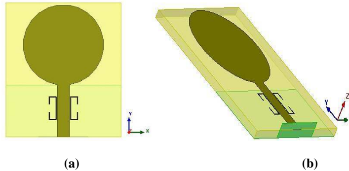
Figure 3: Design of proposed antenna (a) top view and (b) side view of antenna.
