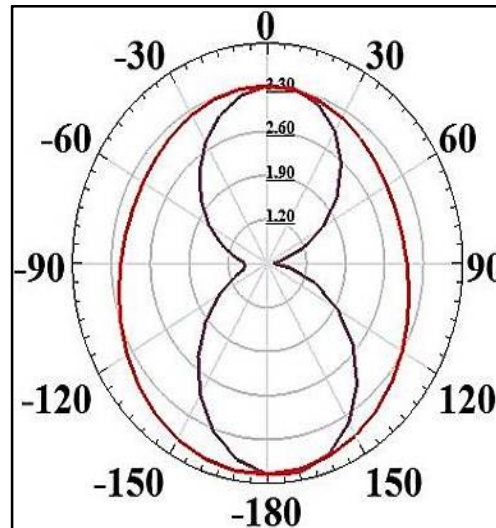
Figure 13: Radiation pattern of E & H plane without SRR loaded.
